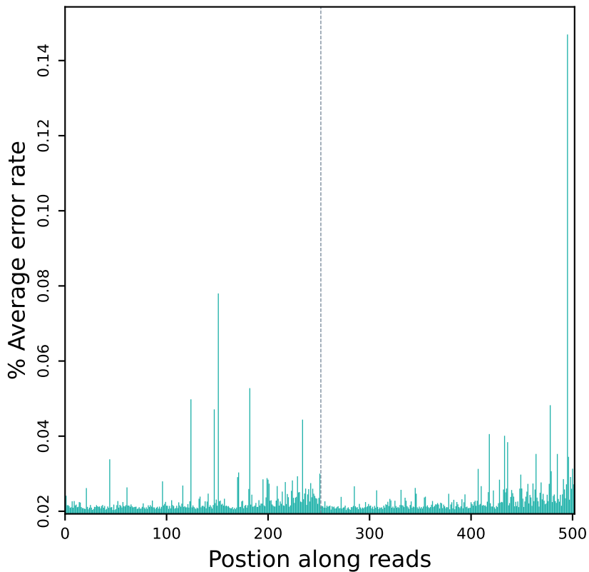
Error rate distribution along reads (R10218)
